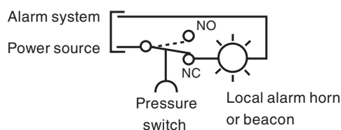
Wiring configuration
